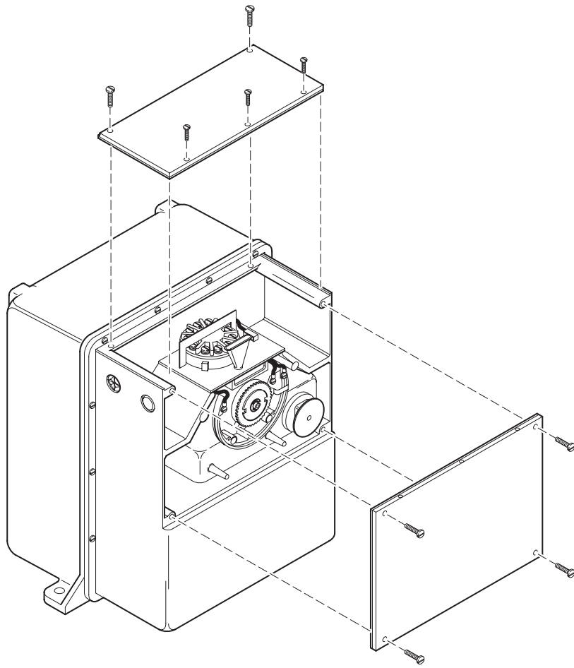
Figure-1 Gasket Cover Kit Used On The MP-9700 Actuator.
