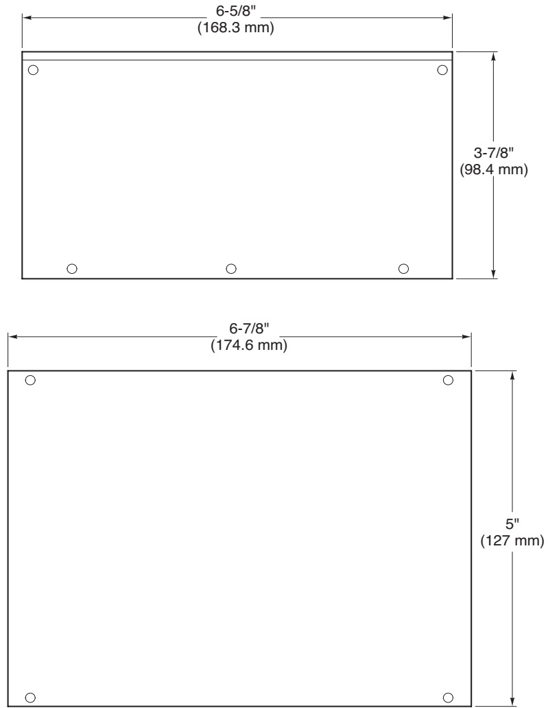
Figure-2 AM-369 Gasket Cover Kit Dimensions.
